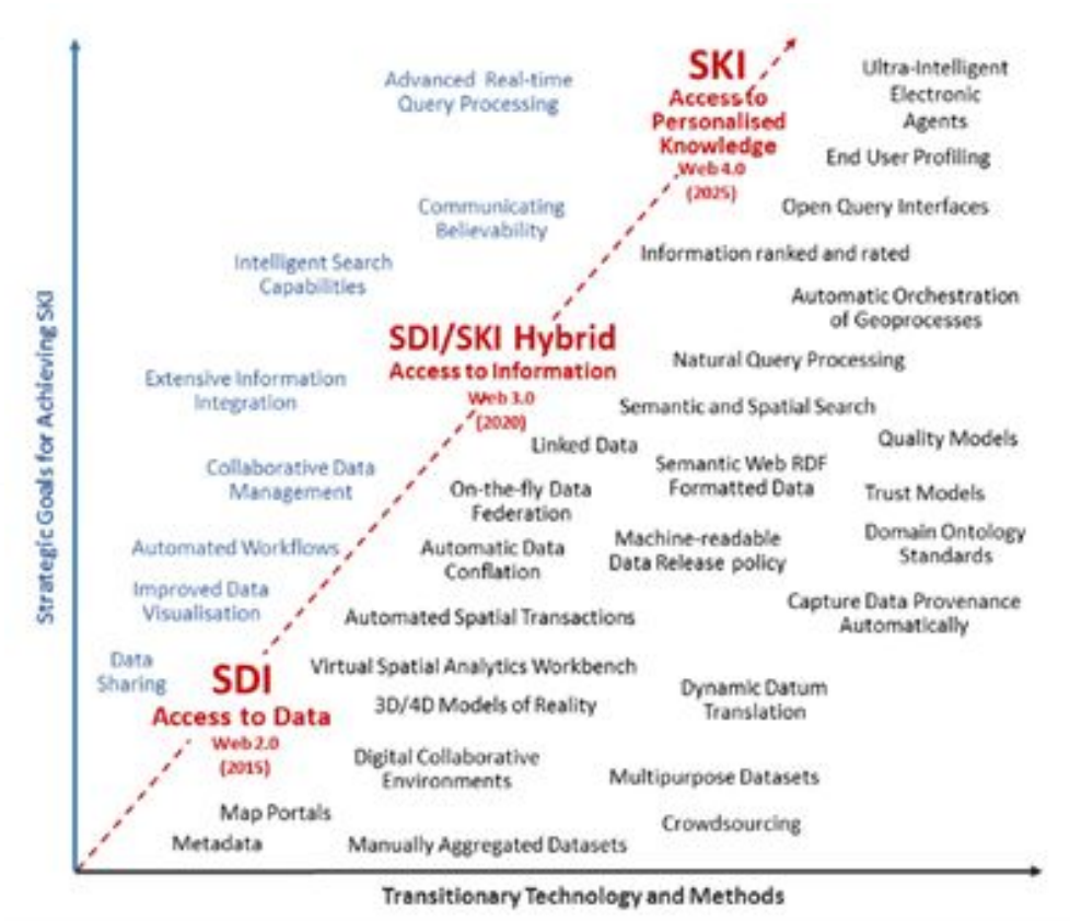
Figura N° 1. La transición de una IDE a una ICE. Fuente: Peter Woodgate et Al. (2017). The Australian approach to geospatial capabilities; positioning, earth observation, infrastructure and analytics: issues, trends and perspectives. Geo-spatial information Science. DOI and URL: http://dx.doi.org/10.1080/10095020.2017.1325612
